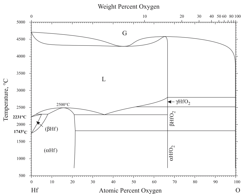
Fig. 1 Hf-O phase diagram
